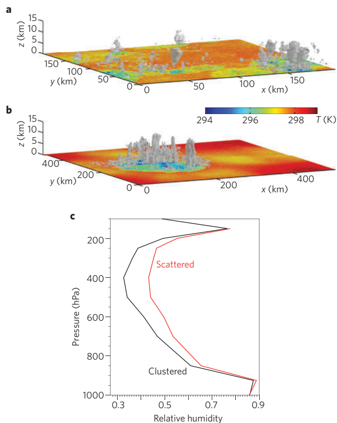
Figure 4 | What role does convective aggregation play in climate? In models, convective organization can exhibit a random distribution (a) or evolve spontaneously towards an aggregated state (b) 42 , increasingly so with increasing temperature 40 . c, In observations (relative humidity profiles from AIRS satellite measurements), the middle troposphere is drier in an atmosphere in which the same amount of precipitation is concentrated in a smaller number of convective clusters 39 . Figure reproduced with permission from a,b, ref. 42, AMS; c, ref. 39, AMS.
