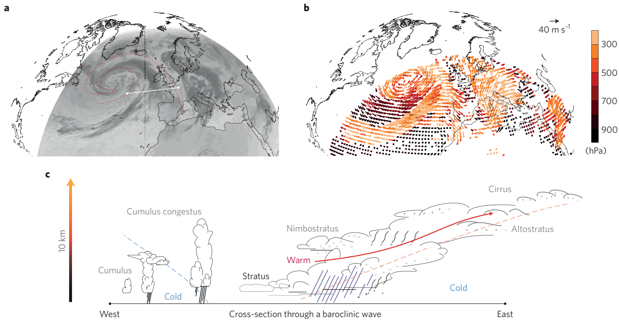
Figure 2 | What controls the position, strength and variability of storm tracks? a , Infrared radiance visualize patterns of clouds in a developing storm whose wavelike structure is outlined by red contour delineating air-mass boundaries in upper troposphere. b , Cloud motion vectors, coloured by cloud-top pressure, derived from radiances. c , Conceptual cartoon illustrating major cloud types along a cross-section through the storm system. In a and b the data are from 5 January 2014 and limited by the field of view of the Meteosat satellite. Panel a,b © 2015, EUMETSAT.
