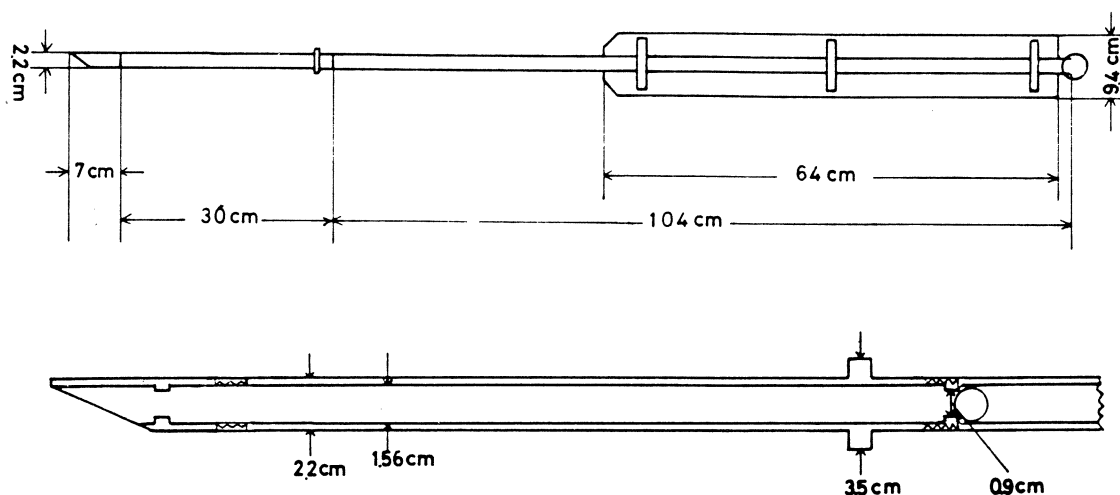
Figure 11.2. Simple gravity coring device designed by the Tokyo University Fisheries Oceanography Laboratory.
