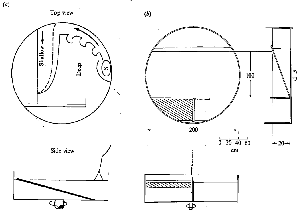
FIGURE 1. The apparatus used to observe the density current over a sloping bottom. (a) Experiment I. The side view shows the false bottom emplaced in the salty water on the turntable. The inverted funnel in contact with the water surface on the right serves as a source of fresh water. The top view shows schematically the shelf, the source (labelled S), and the turbulent gravity current over the shelf. The dashed line is the intersection of the edge of the current with the bottom and the solid line is the intersection with the surface. (b) Experiments II, III. The cross-hatch denotes dyed fresh water of depth H floating above clear salty water. The short dashed line represents the removed sliding gate. The long dashed line is the extra offshore wall in experiment III. The vertical scale has been exaggerated by a factor of two.
