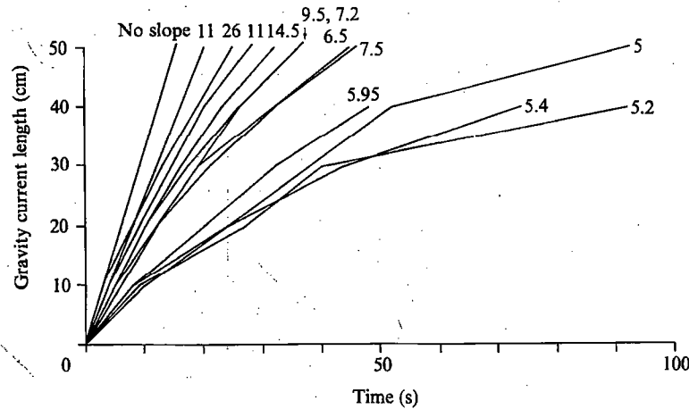
FIGURE 2. Position of the nose of the gravity current with time for the twelve runs in experiment I (from table 1). Trajectory of the gravity current along the vertical wall (no slope) is also shown. The number at the end of each curve corresponds to the rotation period of the tank in seconds.
