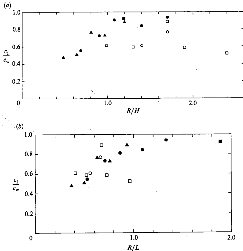
FIGURE 11. Ratio of the initial velocity over the sloping bottom ( c_i ) and the velocity next to the vertical wall ( c_w ) vs. (a) hydrostatic number, R/H and (b) ratio of Rossby radius of deformation to the shelf width R/L (from experiment II). Symbols represent different Reynolds numbers: \blacksquare , Re = 25600 ; \bullet , Re = 8713 ; \blacktriangle , Re = 6161 ; \square , Re = 3200 ; \circ , Re = 2263 .
