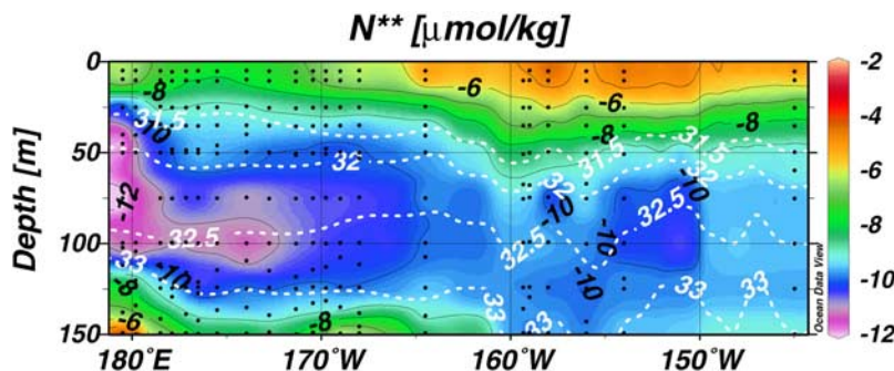
Figure 9. Vertical section of N^{**} from the Chukchi Abyssal Plain in the west to the Canada Abyssal Plain in the east. See Figure 1 for the locations of sampling stations. At each station, data sampling levels are indicated by black dots. The N^{**} contours are from -12 to -5 \mu\text{mol/kg} , with an interval of 1 \mu\text{mol/kg} . White dotted lines indicate salinity contours of 31.5 , 32 , 32.5 , and 33 .
