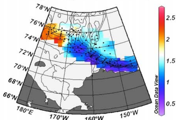
(b) Silicate [ \text{mol}/\text{m}^2 ] from 0 m to S = 33.5
