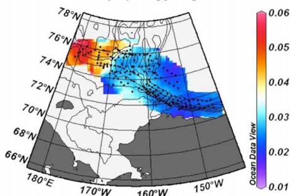
(c) Chlorophyll a [ \text{g}/\text{m}^2 ]
