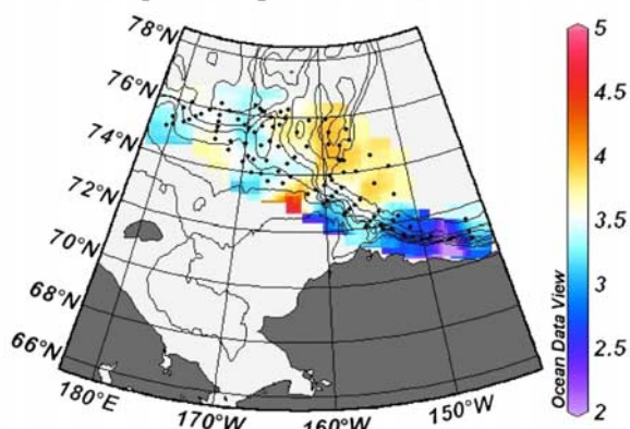
(c) Chlorophyll a [ \text{g}/\text{m}^2 ]
